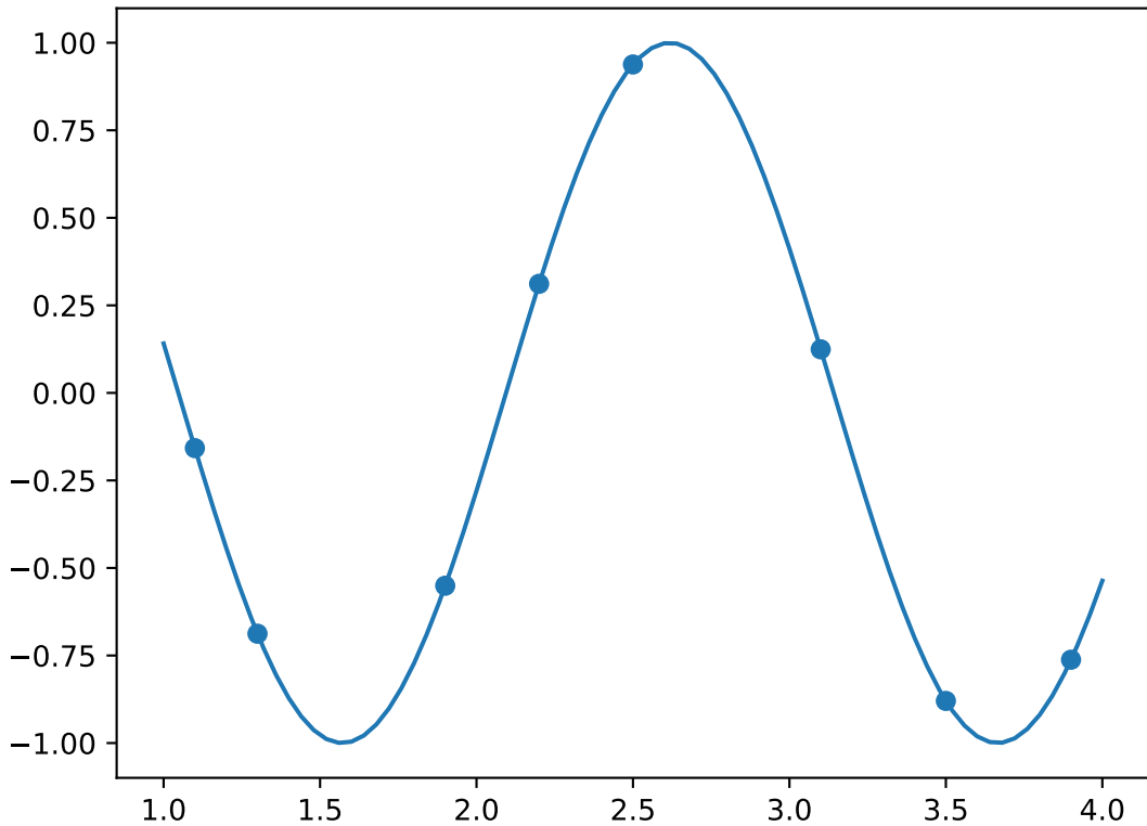
Function to approximate and some specific data sites
